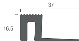
MB18EJ Expansion Strip
